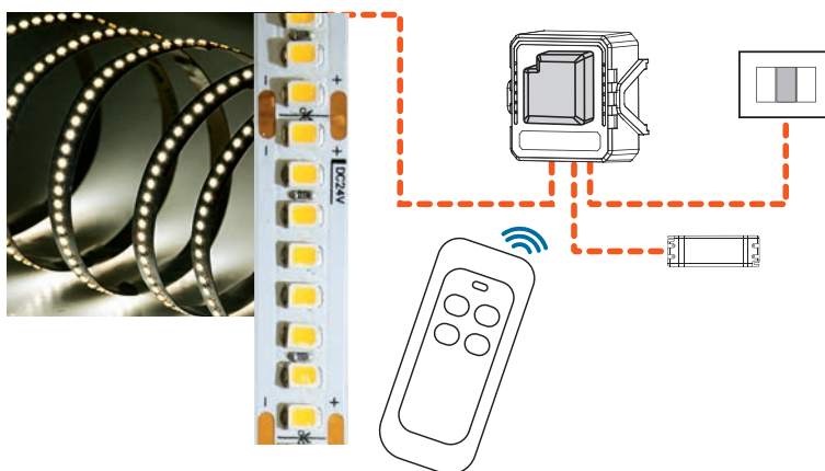
Schema collegamento STRIP LED
